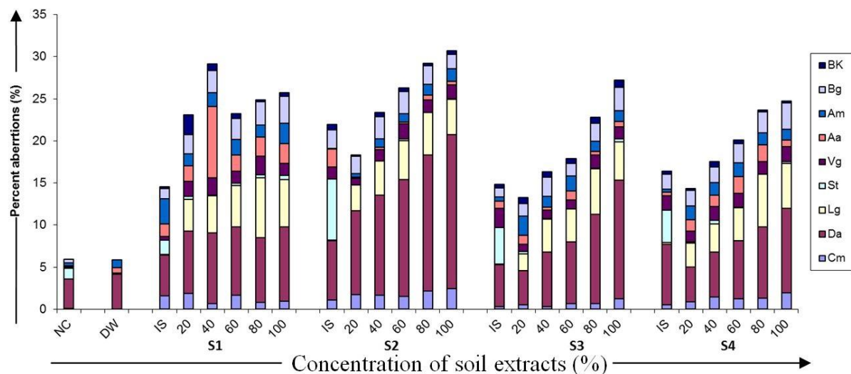
Figure 2. Percent aberrant cells in Allium cepa root tips following in situ and root dip treatment.
